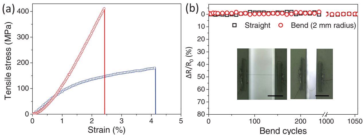
Figure 2. Mechanical and electrical properties of graphene fibers. (a) Typical stress-strain curves of single as-prepared (blue square) and 800 °C thermally treated (red circle) graphene fiber. (b) Electrical-resistance change of a graphene fiber upon repeated bending to a radius of 2 mm and then straightening for over 1000 cycles. The inset photographs show the straight and bending status of a graphene fiber (scale bars = 1 cm).
